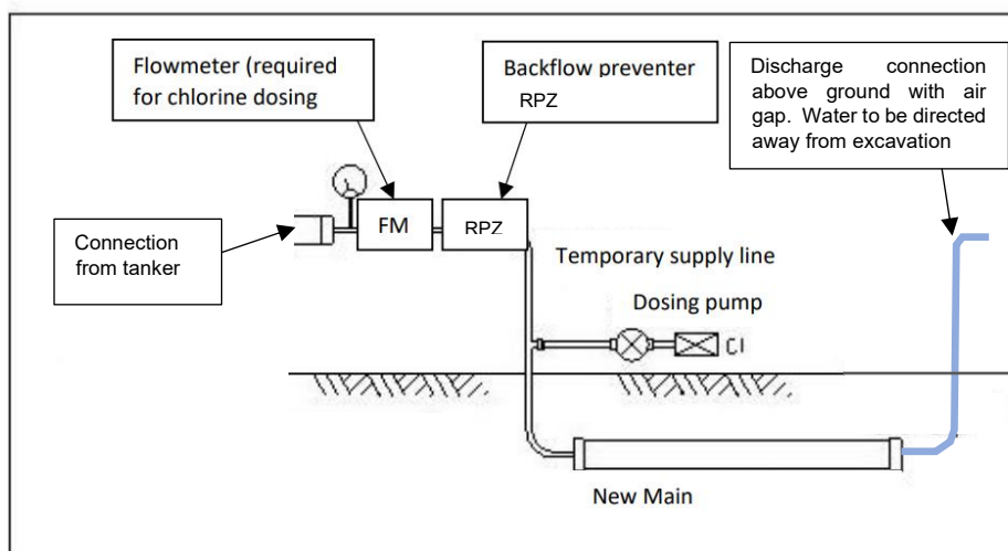
Figure 7.1: Suggested temporary dosing/discharge connection
